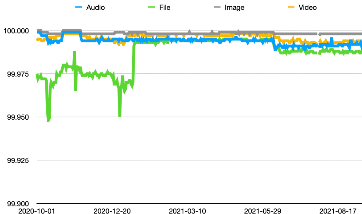
Figure 1: Transport encryption deployment status
